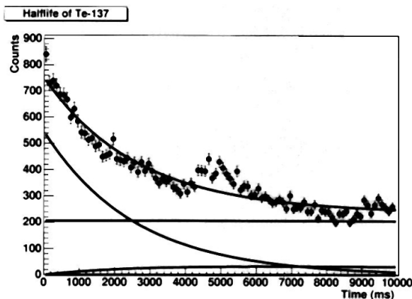
Figure 1: Decay curve of all data from isotope 137 Te.
