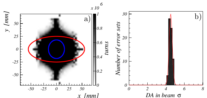
Figure 1: a) Stability domain; b) DA for a beam with \epsilon_{rms,x,y} = 8.75 mm mrad as function of bend errors.
