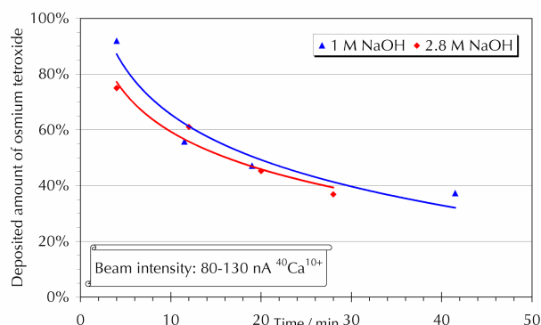
Fig. 1: Deposition of \text{OsO}_4 using unmoisturized gases
