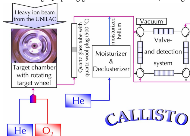
Fig. 2: Scheme of the CALLISTO-setup
