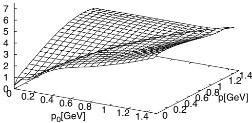
100 Re \Sigma [GeV 2 ]
