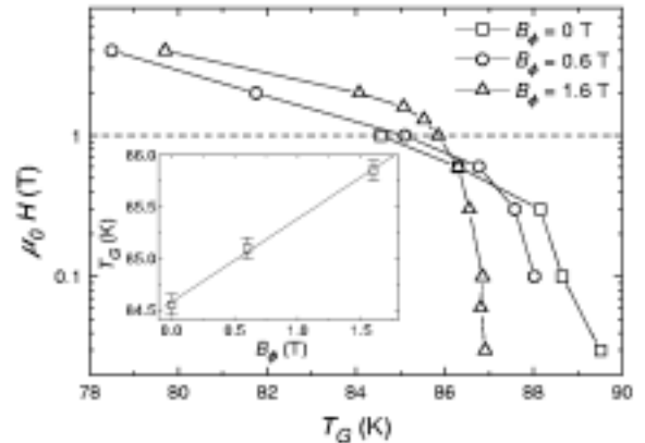
Figure 1: Irreversibility line before and after heavy ion irradiation. For B_0 = 0 T the glass temperature is determined using VG scaling, whereas the BG model is used for the irradiated sample. The number of coherent pinning centers is increased and the (H, T_G) -line is shifted. The insert shows the linear dependence between B_0 and T_G for a magnetic field \mu_0 H = 1 T.
