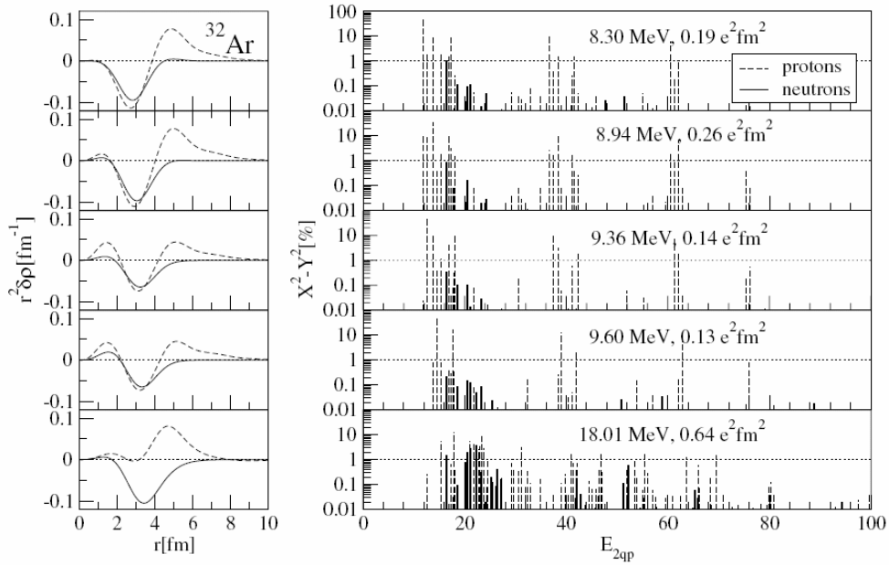
Fig. 2: Proton and neutron transition densities (left panel) and RQRPA amplitudes as a function of the unperturbed energies of 2q\text{p} configurations (right panel) for selected I states [Paa-05b]. The lowest panel is for that a state in the giant dipole regime at 18.01 MeV, the upper panels for states in the energy regime of the pygmy resonance (8.3 – 9.6 MeV).
