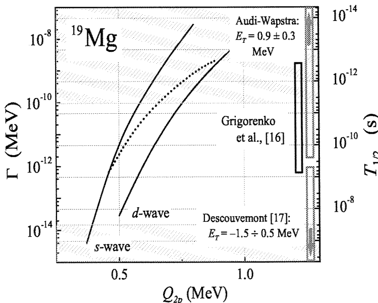
Figure 2: Width and half-life (right ordinate) versus the 2p -decay energy of ^{19}\text{Mg} . The solid curves are the three-body model predictions assuming different l^2 components dominating in the nucleus. Dotted curve takes into account the correct Coulomb displacement energy for a structure with mixed components. The upper hatched area corresponds to the half-lives which are too short for the decay-in-flight experiment (e. g. T_{1/2} less than \sim 5 ps), the lower hatched area corresponds to the long half-lives suited for an implantation.
