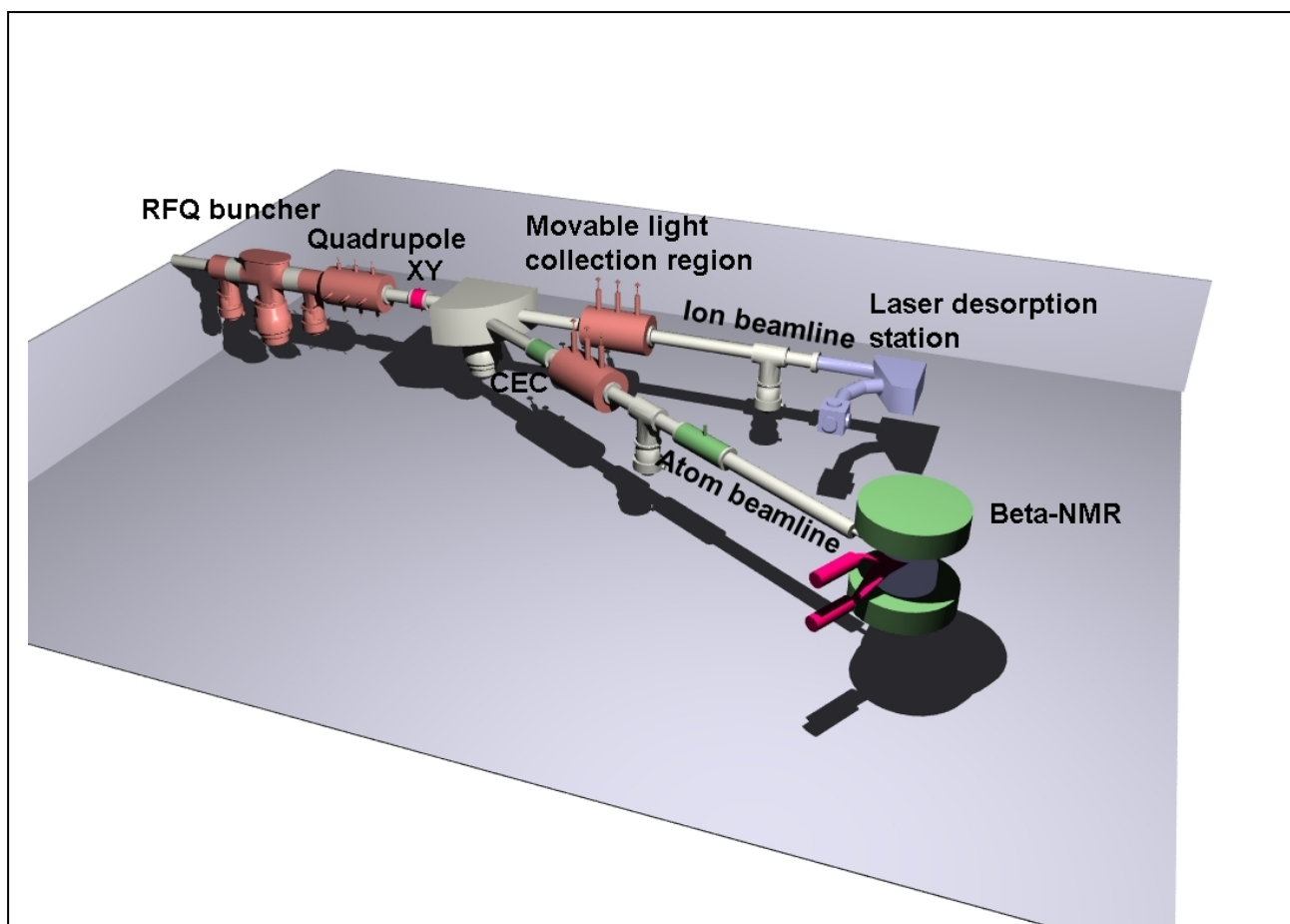
Figure 1: Overview of the proposed LaSpec set-up including RFQ buncher, collinear ion spectroscopy, collinear atomic beam spectroscopy and optical pumping, laser-desorbed resonance ionization and \beta -NMR.
